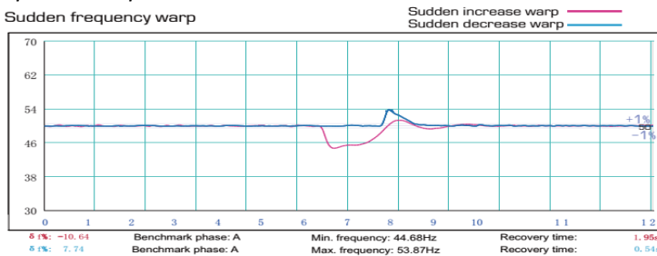
Sudden frequency warp
